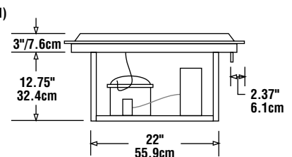
RIGHT END VIEW N8200 MODELS
