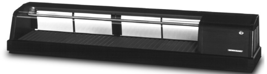
HNC-150AA-R(L) W x D x H 59.1" x 13.6" x 11"
