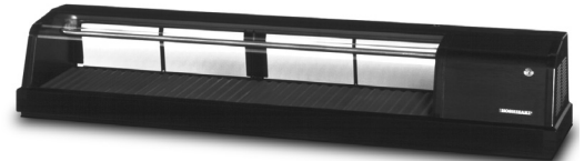
HNC-150AA-R(L) W x D x H 59.1" x 13.6" x 11"
